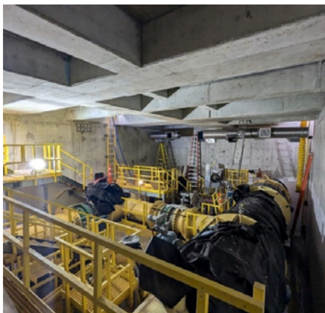
Figure 15: Kennedy Newton Water Main – Installation of Piping and Valves within the Large Underground Valve Chamber
