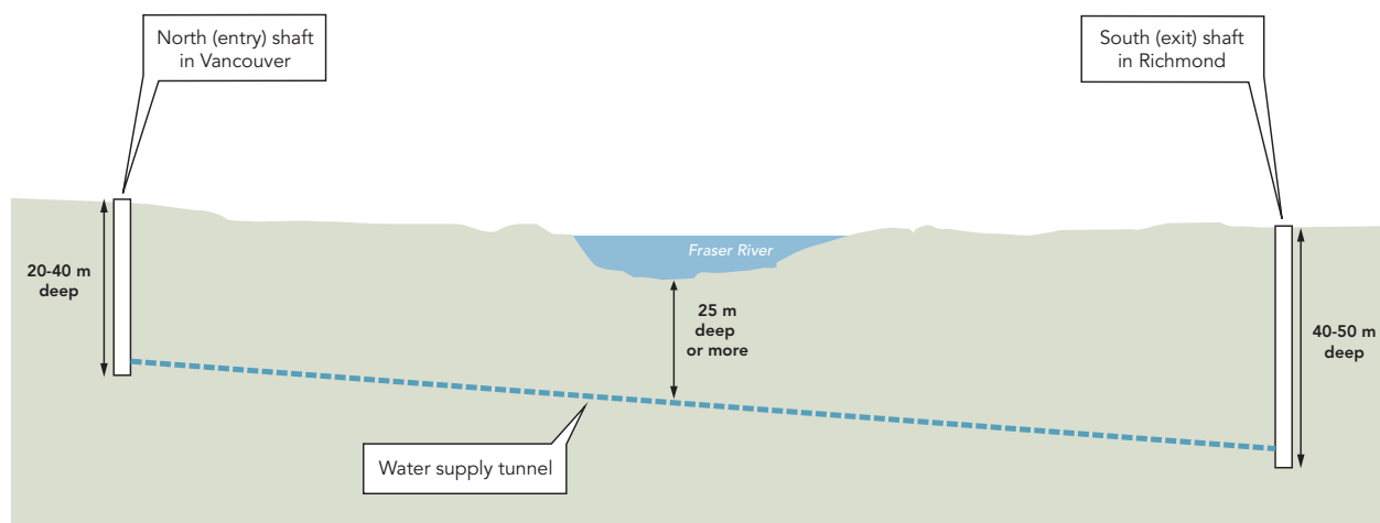
CAMBIE-RICHMOND WATER SUPPLY TUNNEL – Cross section
