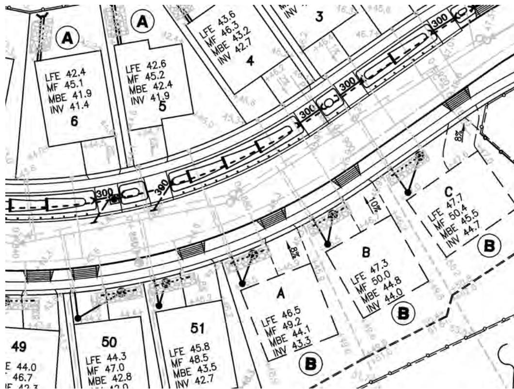
Figure 1D: Example of Engineering Plan (Silver Ridge – KWL Associates Ltd.)
