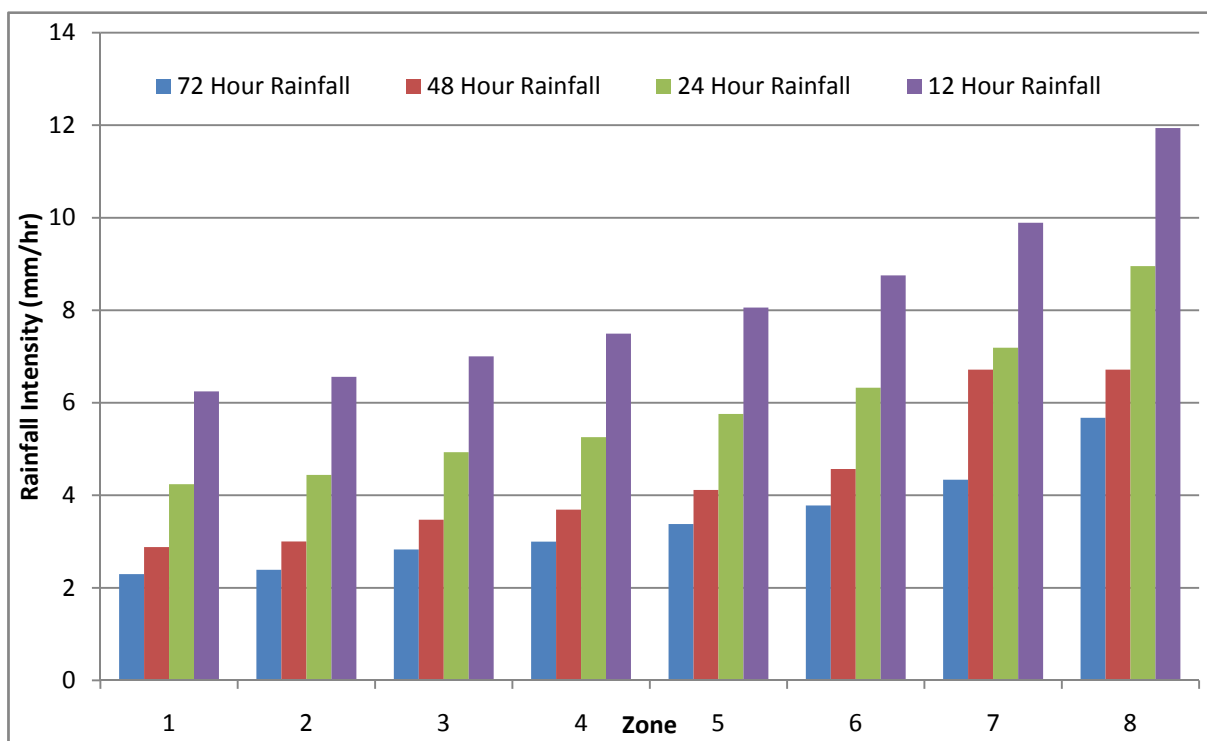
Figure 3-1. 12 to 72-hour, 100-year rainfall intensities, Zones 1-8.
