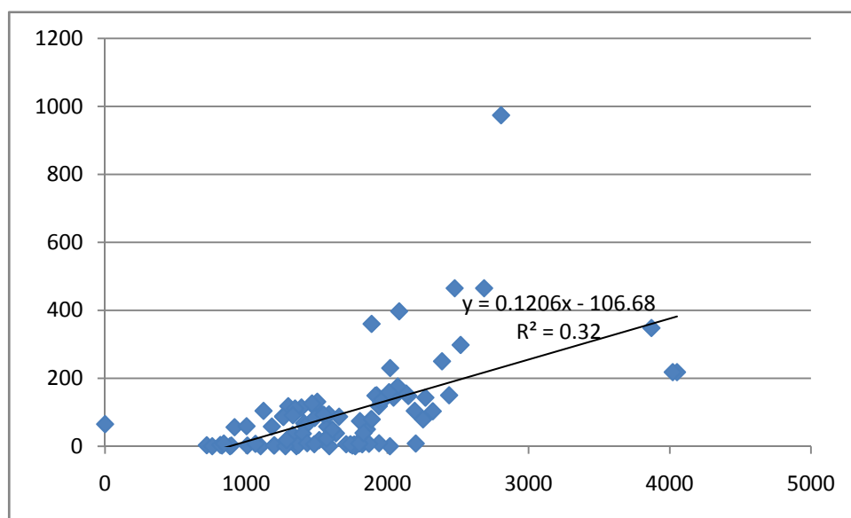
Figure 4-1. Elevation plotted with Average Annual Precipitation.
