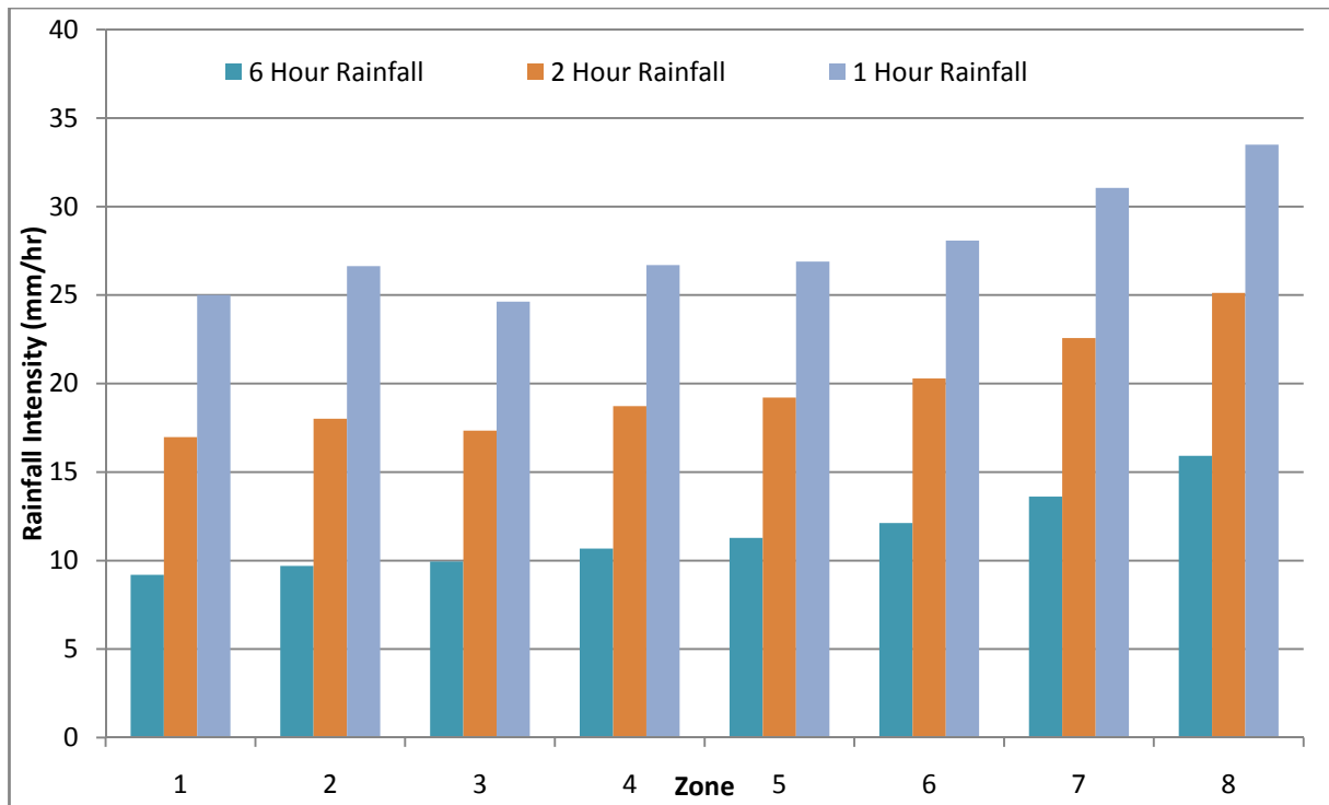
Figure 3-2. One to 6-hour, 100-year rainfall intensities, Zones 1-8.
