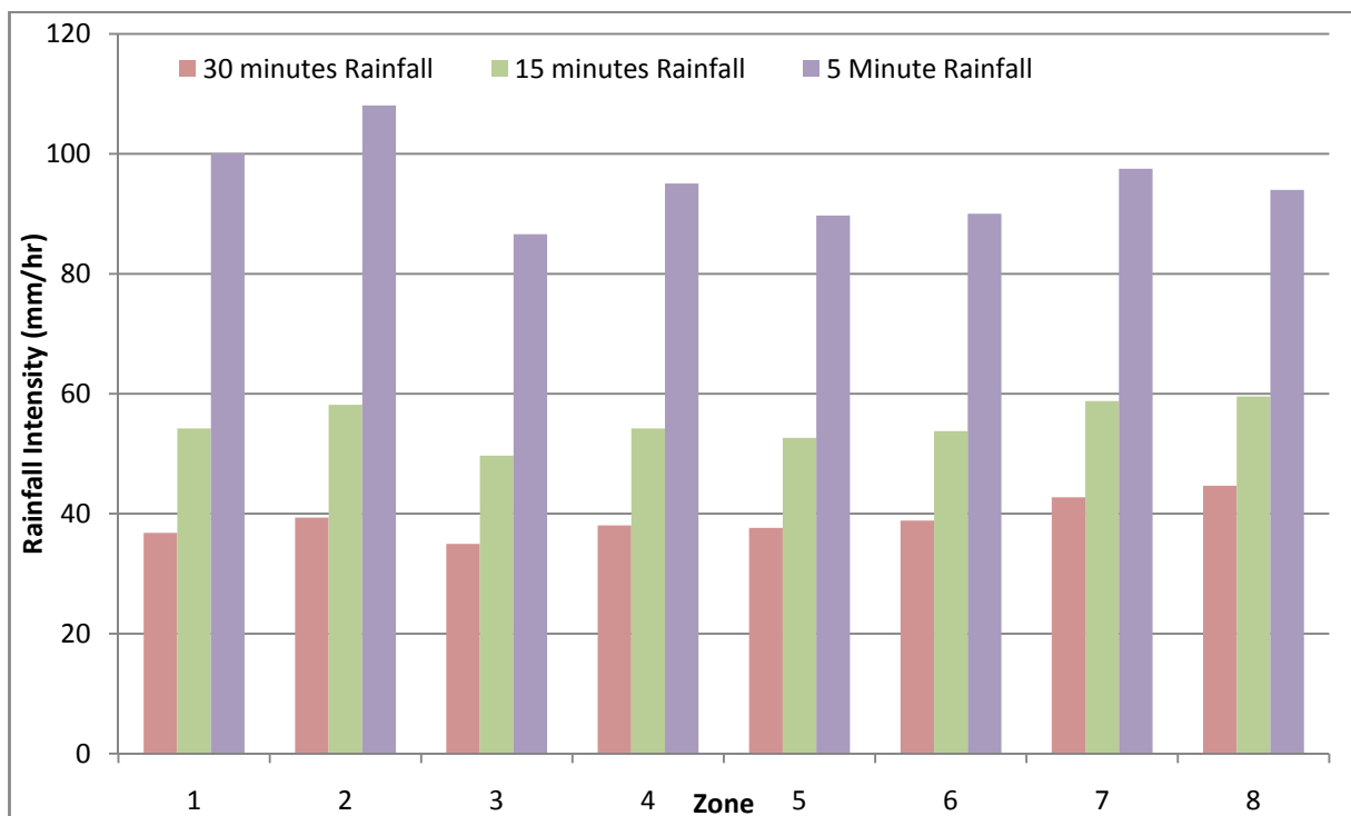
Figure 3-3. Five minute to 30 minute, 100-year rainfall intensities, Zones 1-8.
