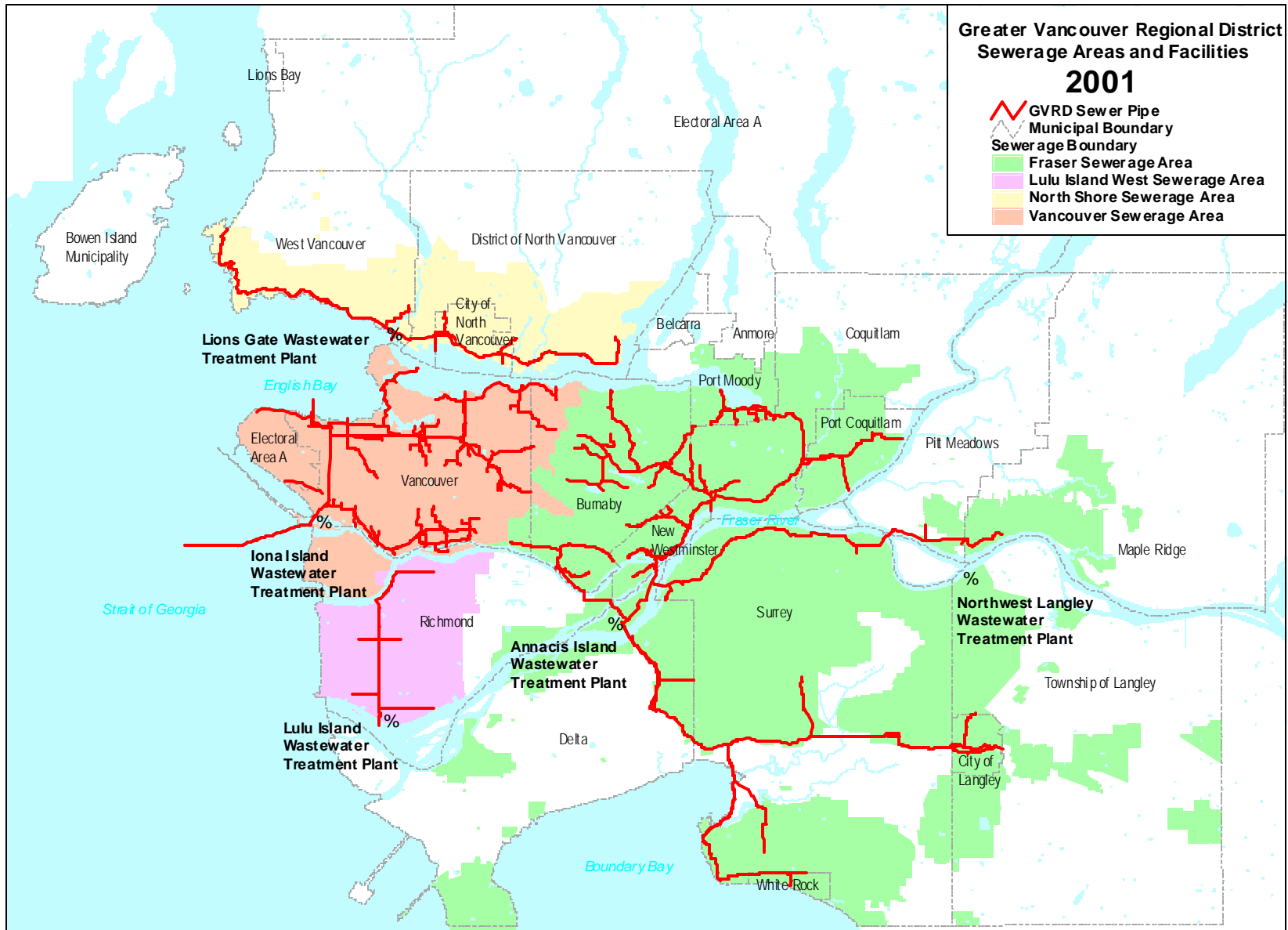
Figure 2: GVRD Municipalities and Sewerage Areas/Facilities
